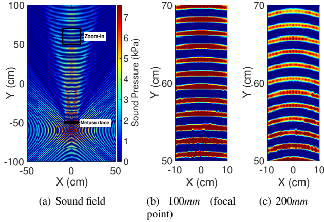
Figure 4: (a) Sound field simulated in COMSOL with a 16 \times 1 metasurface when we transmit 20\text{kHz} sound at the focal point ( 100\text{mm} ). Part of the energy is concentrated in a specific direction. (b) and (c) show the sound field in the zoom-in area when the speaker is placed at 100\text{mm} and 200\text{mm} , respectively. When the speaker is at the focal point, the signal coming out of the lens is a parallel wave.
