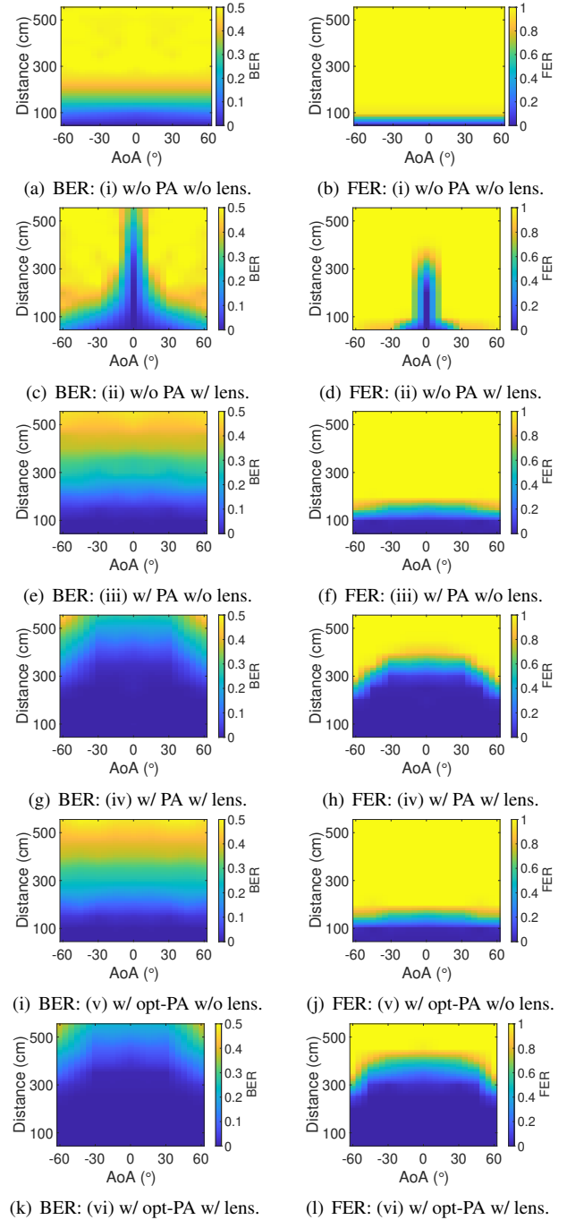
Figure 24: The impact of distance and AoA on the communication performance.
