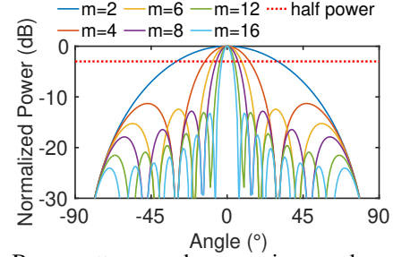
Figure 5: Beam patterns under a varying number of speakers m . The received sound is normalized by dividing it by the maximum power and then converted to decibels.
