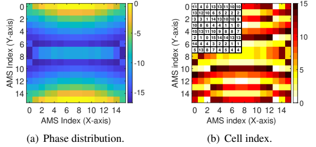
Figure 11: Phase distribution and cell indices of the optimized 16 \times 16 lens design, where the cell index is the index to one of the 16 quantized phase shifts. The numbers in the upper left corner denote the cell indices for the top left metasurface and we omit the other parts for brevity due to the left-right symmetry and top-bottom symmetry.
