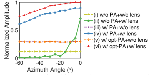
Figure 14: Power gain while steering at various angles. The amplitude is normalized by dividing it by the maximum amplitude of scheme (vi). The testbed uses a 16 \times 16 acoustic lens and 6 speakers to form a phased array.
