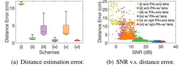
Figure 19: The distance estimation performance using acoustic lens.
